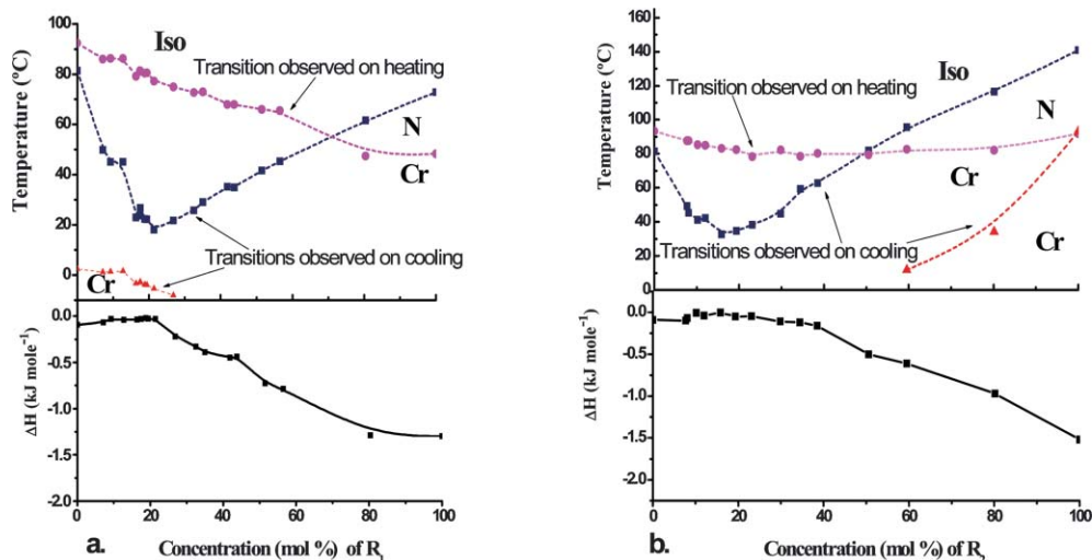
Fig. 5 Phase diagrams of (a) D_2 - R_1 , (b) D_2 - R_2 . The upper plots refer to the mixtures of discs and rods as determined by DSC measurements. The compositions are plotted as molar concentrations of the rods. Data shown in magenta refer to enantiotropic N-I transitions obtained on heating; data shown in blue refer to N-I transitions recorded on cooling. Data shown in red indicate crystallisation temperatures recorded on cooling. Glass transitions are omitted. The sketched lines are guides for the eyes only. The lower plots refer to the enthalpy changes associated with the N-I transitions recorded on cooling.
