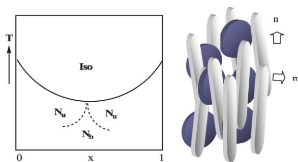
Fig. 1 Schematic phase diagram containing the N_b phase for mixtures of rods and discs. x represents the fraction of discs. The shape of the phase diagram, especially the transitions between the N_b and the N_u phases, is actually dependent on the model used. n and m refer to the two nematic directors in the biaxial phase.
